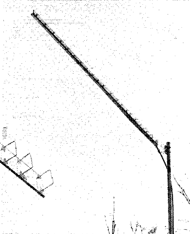
Fig. 3 — The largest quagi tested on 1296 MHz. This 25-element model is built on two tapered 7-ft (2.1-m) lengths of Plexiglas that form a right angle for additional mechanical stability. In case you're thinking of building one like it for the 20-meter band instead of 23 centimeters, the boom length will be a mere 650 ft (198 meters)!
