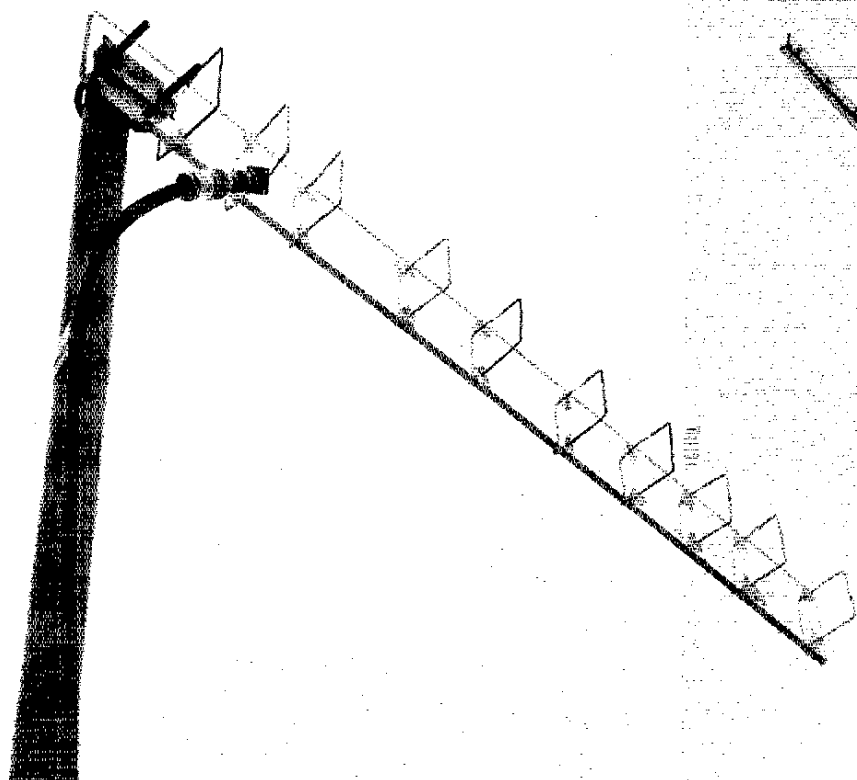
Fig. 2 — This 10-element cubical quad is virtually identical in performance to the 10-element quagi. A 3- x 30-in. (76- x 760-mm) sheet of Plexiglas supports the elements, which are offset slightly to allow room for the feed point on the driven element. All elements are made of insulated no. 18 AWG solid-copper wire.
